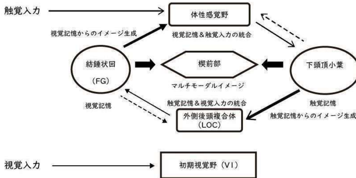
Brain function mechanism of object recognition in 3D shape (Nishino, 2008)
